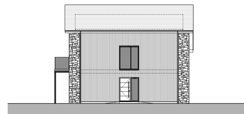
FRONT (ENTRANCE) 1:200
